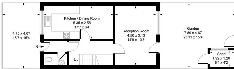
Ground Floor
