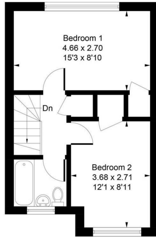
Third Floor
