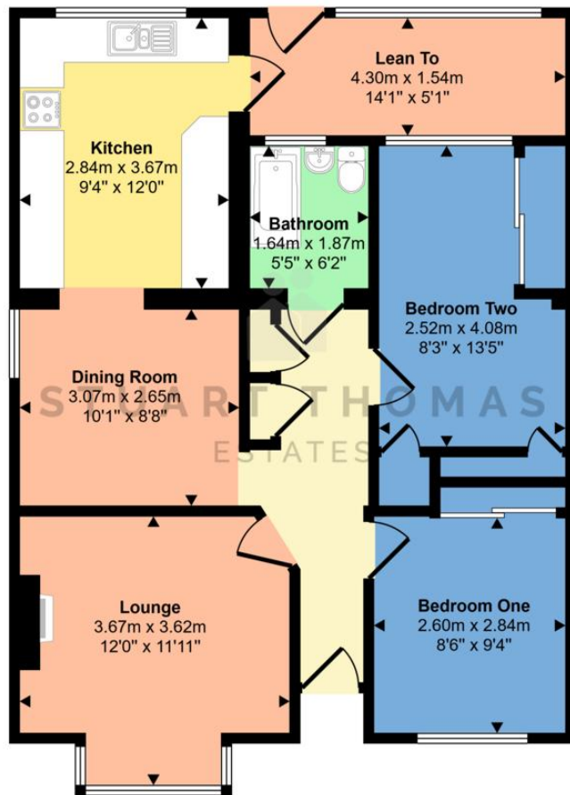
Floorplan
