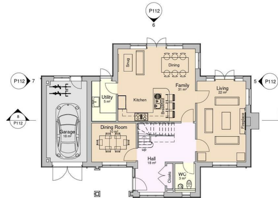
1 0.01 Ground Floor Plan 1 : 100
