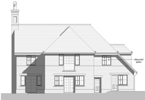
6 Rear Elevation 1 : 100
