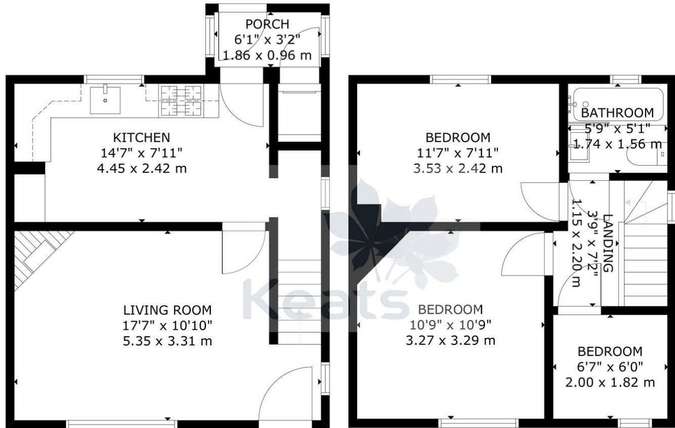
GROUND FLOOR
