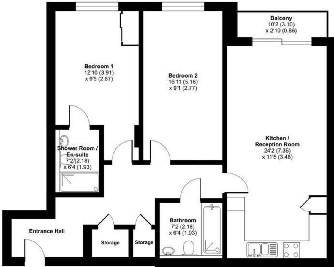
FIRST FLOOR
