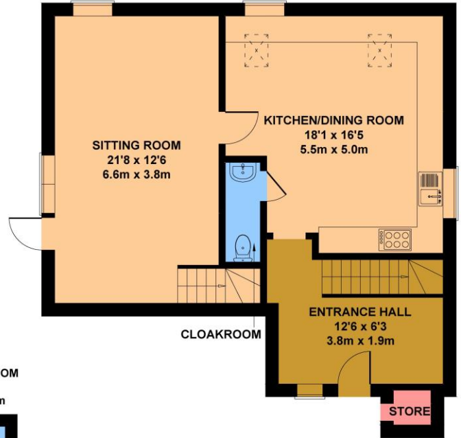
GROUND FLOOR APPROX. FLOOR AREA 720 SQ.FT. (66.9 SQ.M.)
