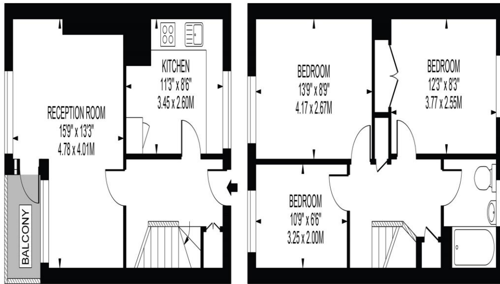
SECOND FLOOR
