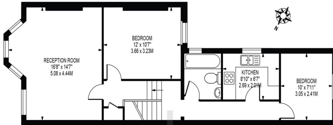
FIRST FLOOR
