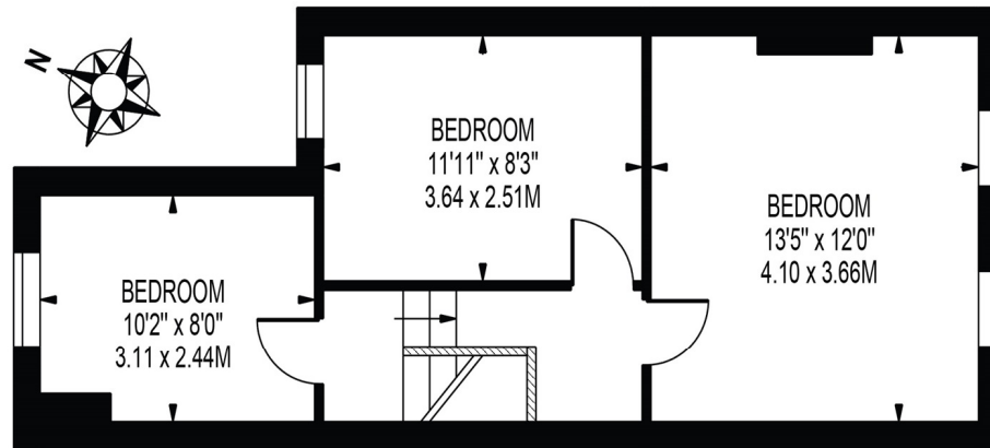
FIRST FLOOR
