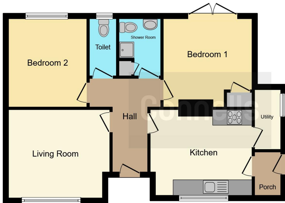
Floor Plan
