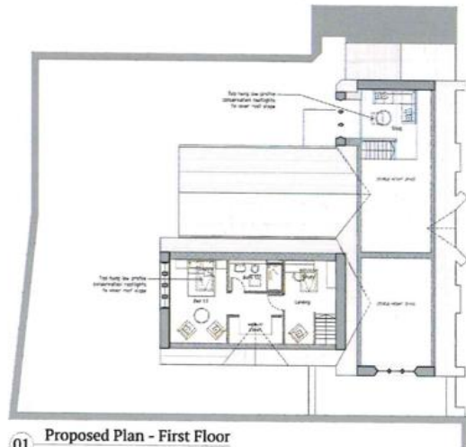
01 Proposed Plan - First Floor 1:100
