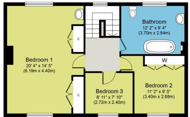
First Floor Approximate Floor Area 680 sq. ft. (63.1 sq. m.)
