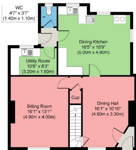
Ground Floor Approximate Floor Area 806 sq. ft (74.87 sq. m)
