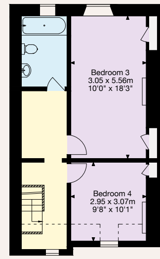
Third Floor
