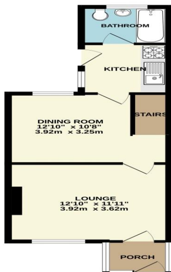
GROUND FLOOR 403 sq.ft. (37.4 sq.m.) approx.
