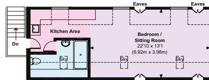
Garage First Floor
