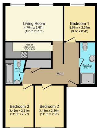
Floor Plan
