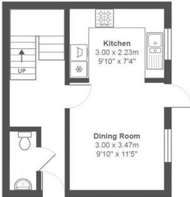
Ground Floor Area: 28.8 m 2 ... 310 ft 2
