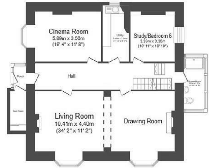
Ground Floor Floor area 122.2 sq.m. (1,316 sq.ft.)
