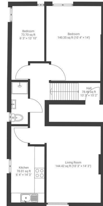
THIRD FLOOR
