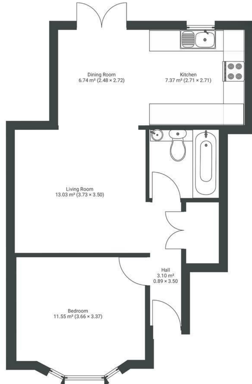
Ground Floor
