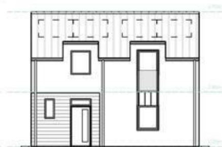
South (street facing) Elevation w/o Gable
