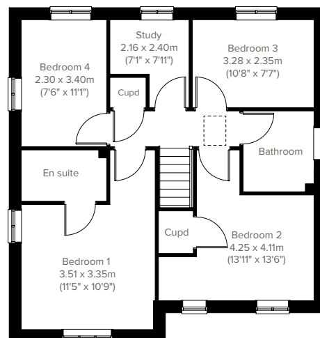
1ST FLOOR
