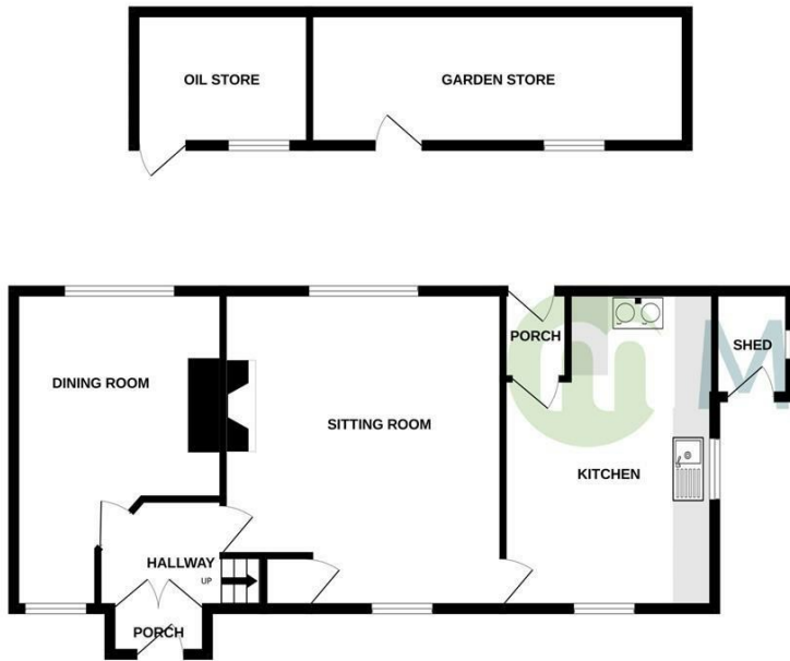
GROUND FLOOR 892 sq.ft. (82.9 sq.m.) approx.
