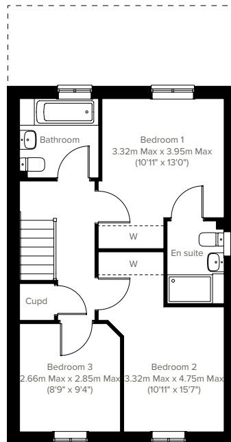
1ST FLOOR
