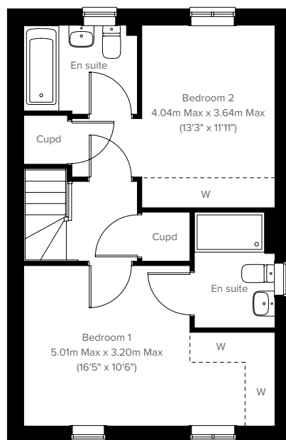
1ST FLOOR
