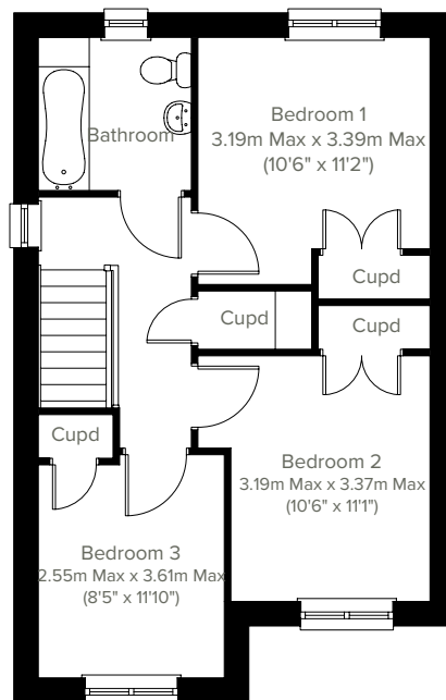
1ST FLOOR
