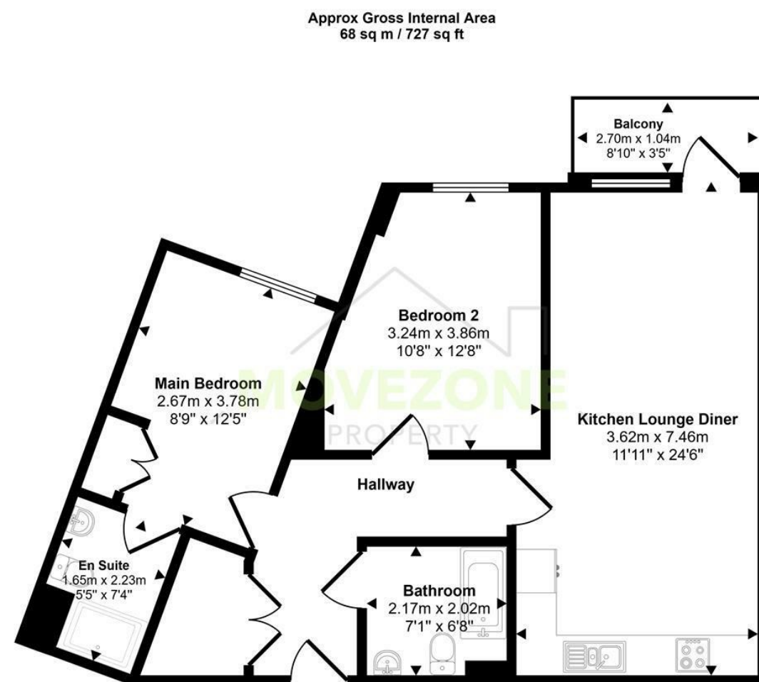
Floorplan
