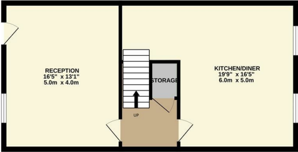
GROUND FLOOR 540 sq.ft. (50.1 sq.m.) approx.
