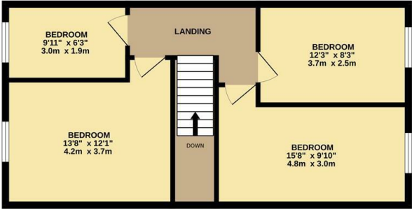
1ST FLOOR 540 sq.ft. (50.1 sq.m.) approx.
