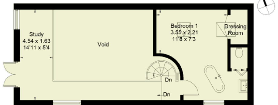
First Floor
