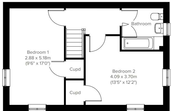
1ST FLOOR
