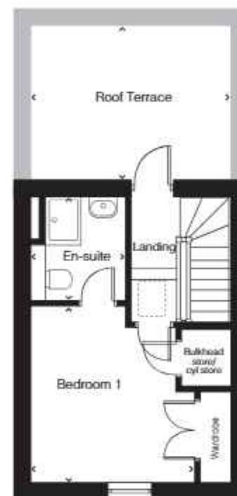
Second Floor
