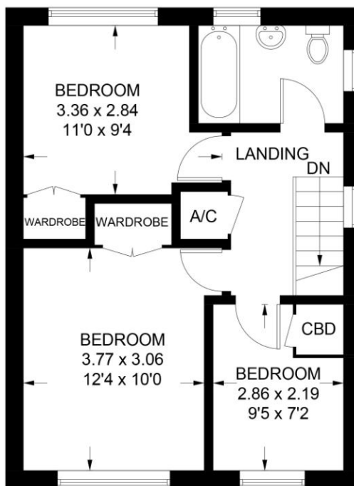
First Floor 40.5 sq m / 436 sq ft
