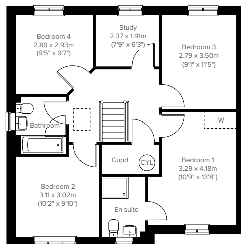
1ST FLOOR
