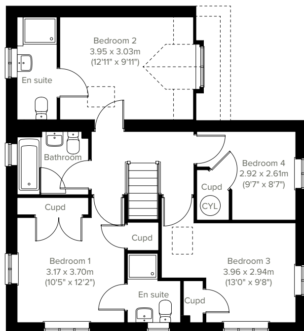
1ST FLOOR
