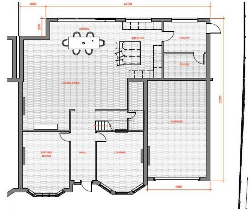
1 GROUND FLOOR PLAN SCALE: 1:50
