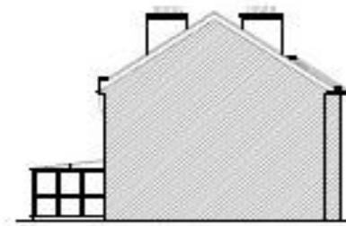
EXISTING ADU SIDE ELEVATION (scale 1:100)
