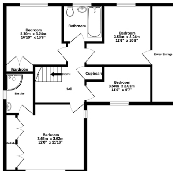
1st Floor 63.0 sq.m. (678 sq.ft.) approx.
