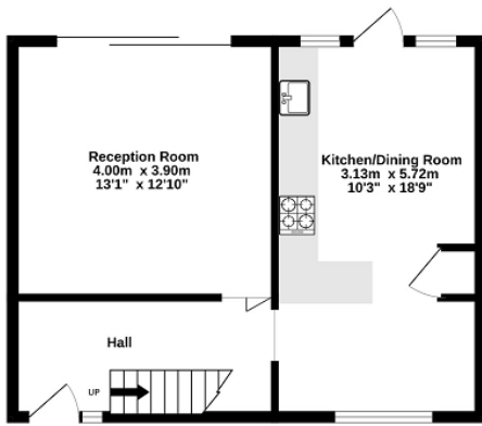
Ground Floor 41.0 sq.m. (441 sq.ft.) approx.
