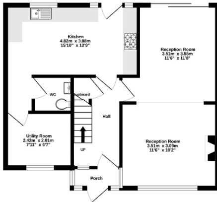
Ground Floor 53.0 sq.m. (570 sq.ft.) approx.
