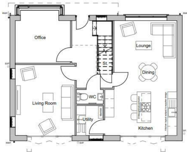
Ground Floor - GA Plan
