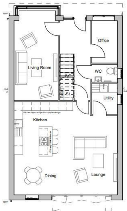
Ground Floor - GA Plan
