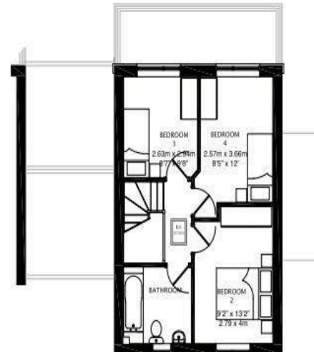
Second Floor Layout
