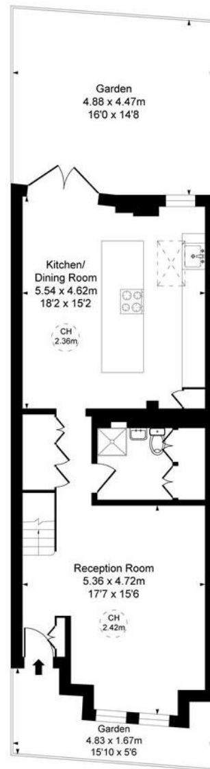
Ground Floor
