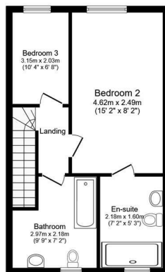
Second Floor Floor area 45.2 m 2 (486 sq.ft.)
