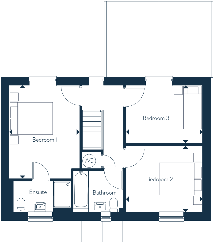
FIRST FLOOR
