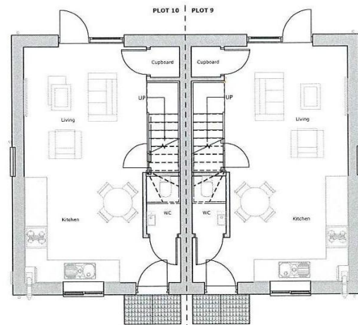
Proposed Ground Floor Plan 1 : 50
