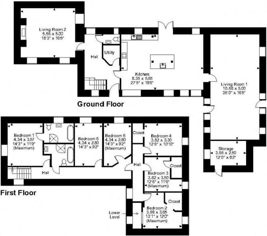
The Old Granary, Rudry, Caerphilly Approximate Gross Internal Area Main House = 3,207 sqft / 298 sq m
