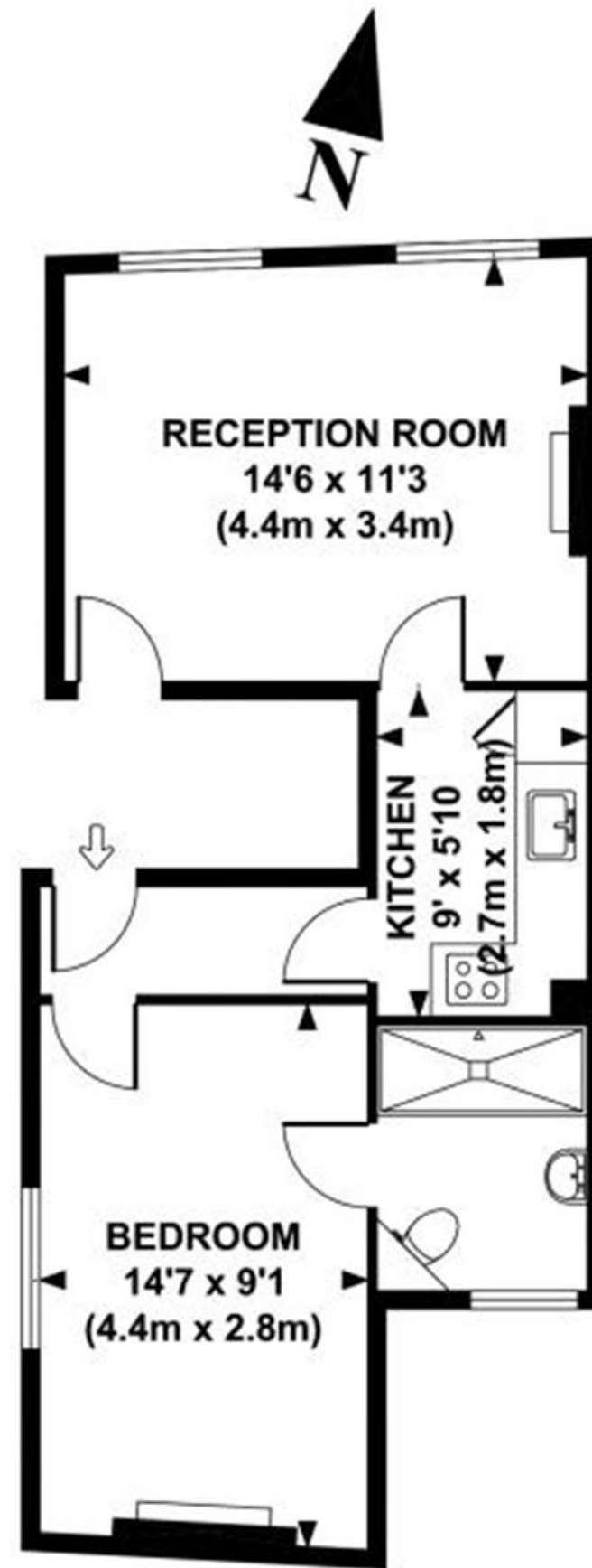
SECOND FLOOR
