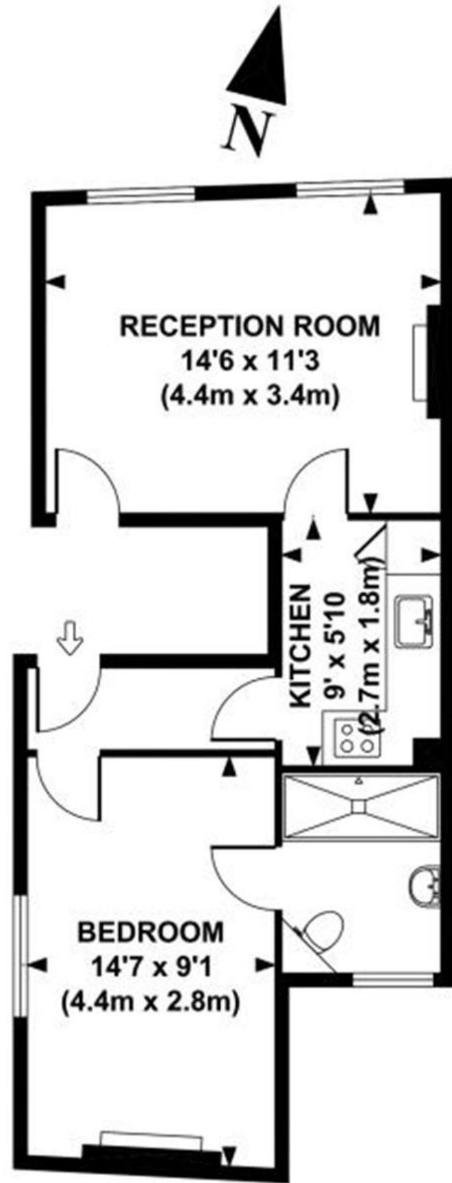
FIRST FLOOR
