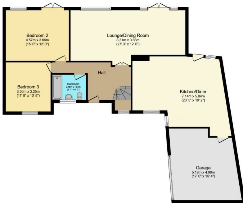
Ground Floor Floor area 130.9 sq.m. (1,409 sq.ft.)
