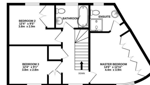
1ST FLOOR 542 sq.ft. (50.3 sq.m.) approx.
