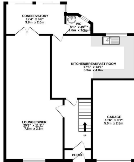
GROUND FLOOR 787 sq.ft. (73.1 sq.m.) approx.
